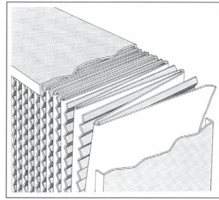
Conventional HEPA construction
